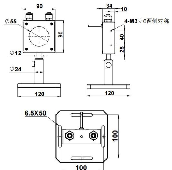
Probe TS700
